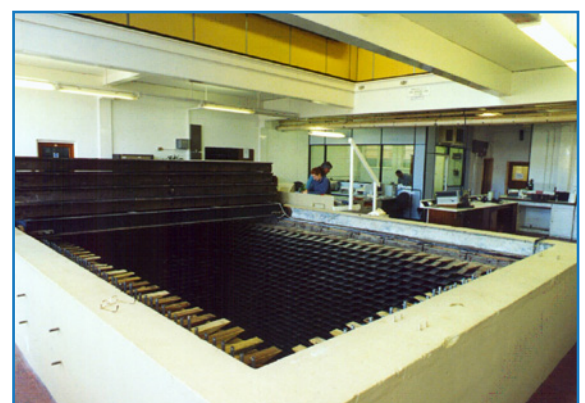
The in-house Acoustic Test Tank hosts a computer-controlled transducer test and calibration facility
